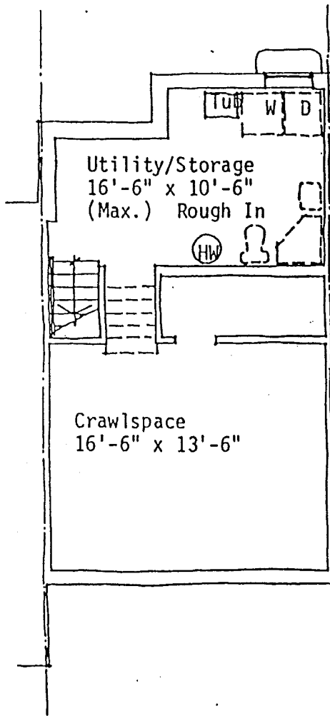
BASEMENT FLOOR PLAN
